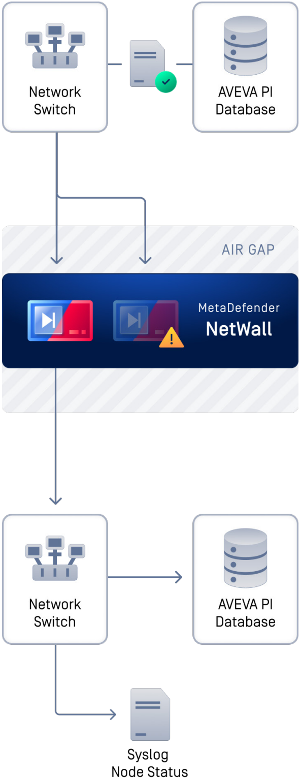
High Availability data flow with MetaDefender USG and BSG
