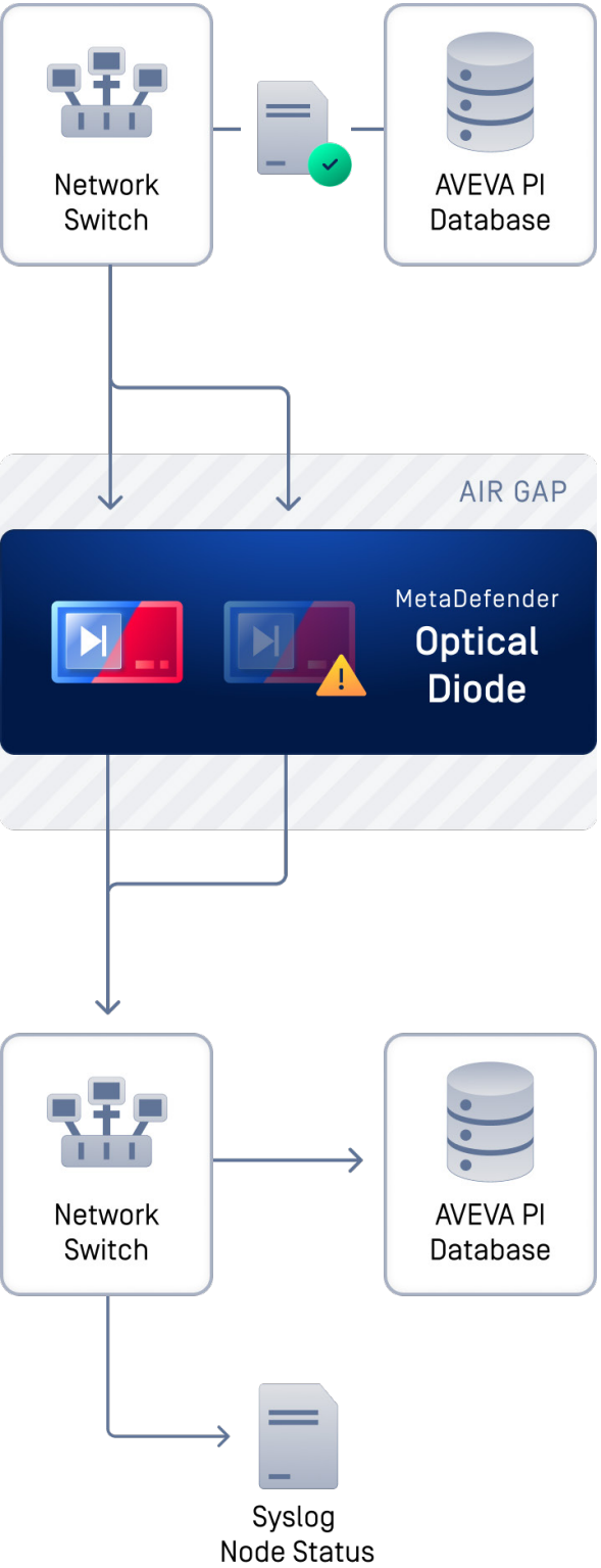
High Availability data flow with MetaDefender Optical Diode
